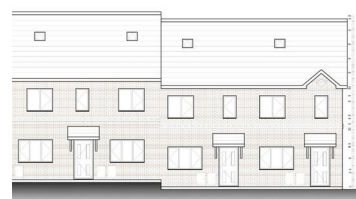
PROPOSED FRONT ELEVATION
